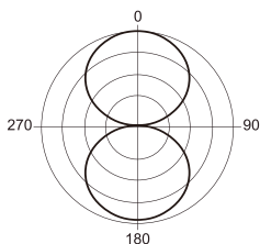
Bidirectional
